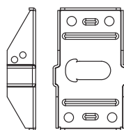
2 Base metallica
